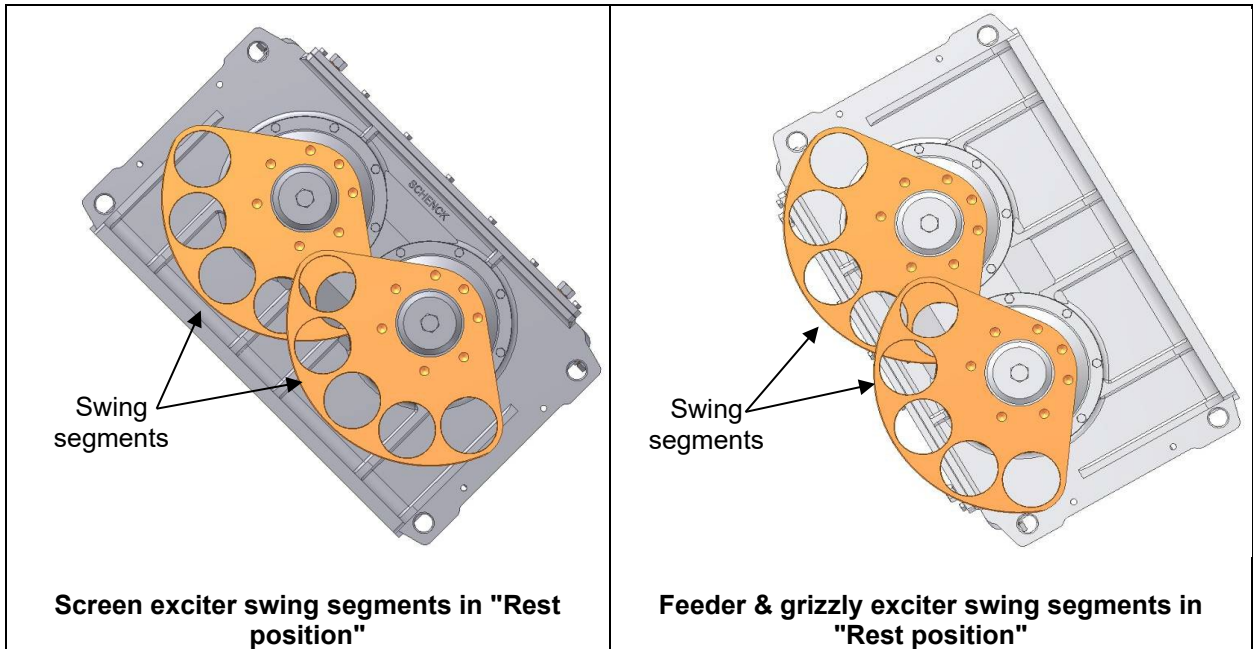
Figure 8.6-1: Exciter swing segment in "Rest position"
