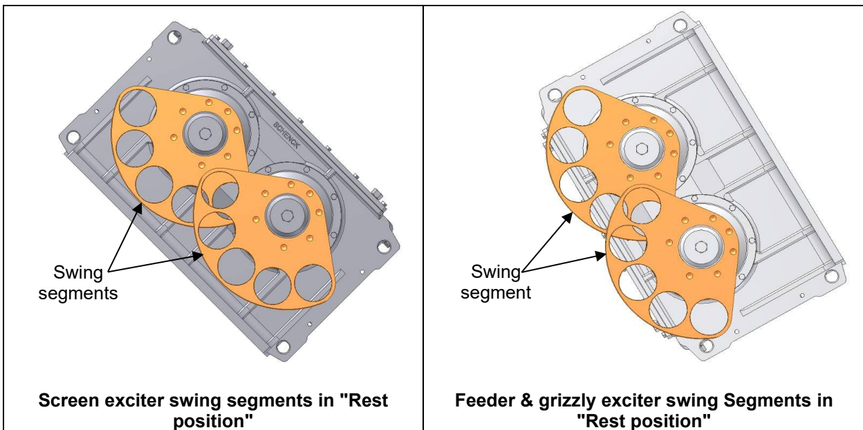
Figure 3.8-1- Exciter swing segment in “Rest position”
