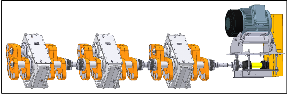
Figure 8.6-4 Example exciter & drive train assembly
